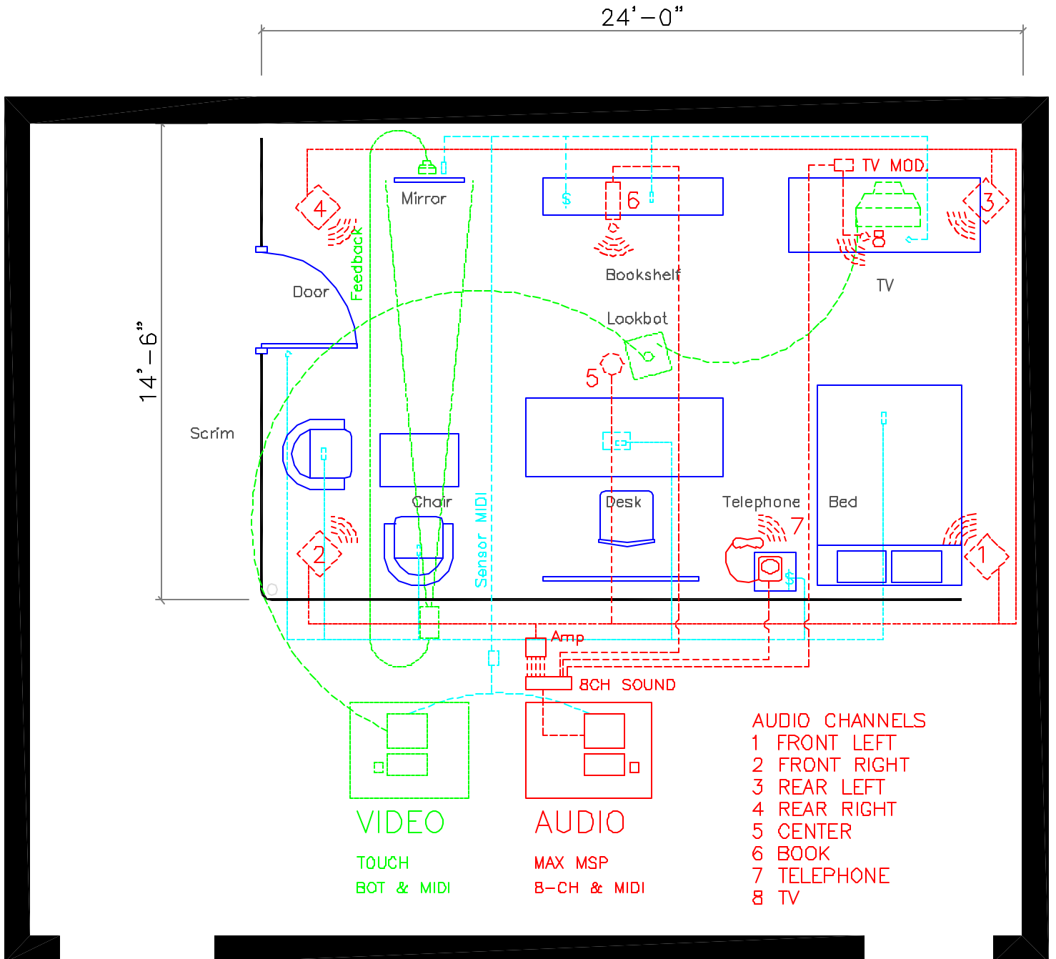
WHITE ROOM PLAN
